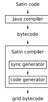
Figure 1. Compiler procedure with automatic sync generation.
