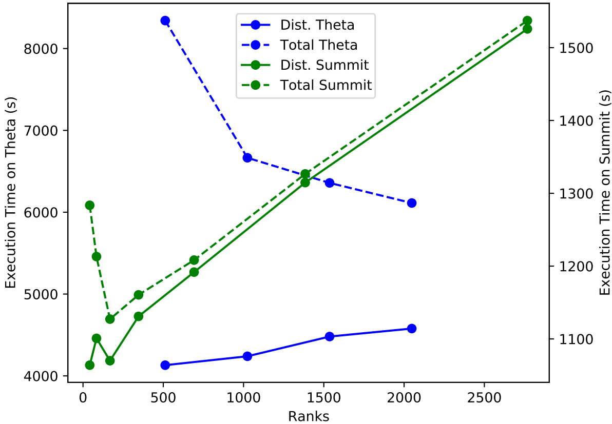
Time to distribute 8K x 8K 2D mesh
