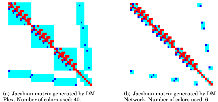
Fig. 3. Comparison of Jacobian preallocation with DMPlex and DMNetwork.
