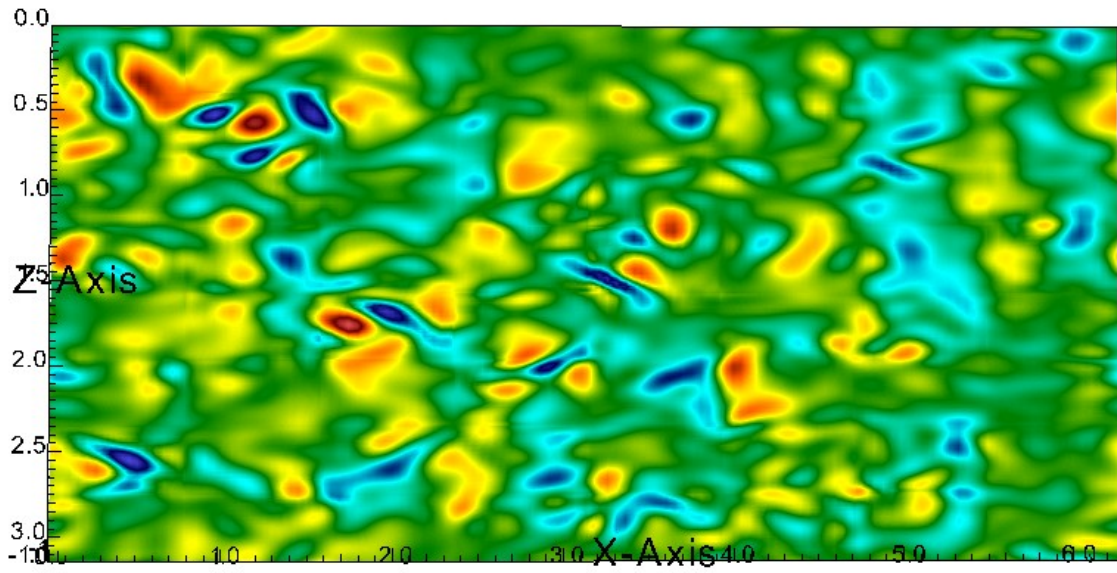
Pressure interpolated from domain-1 to domain-2
